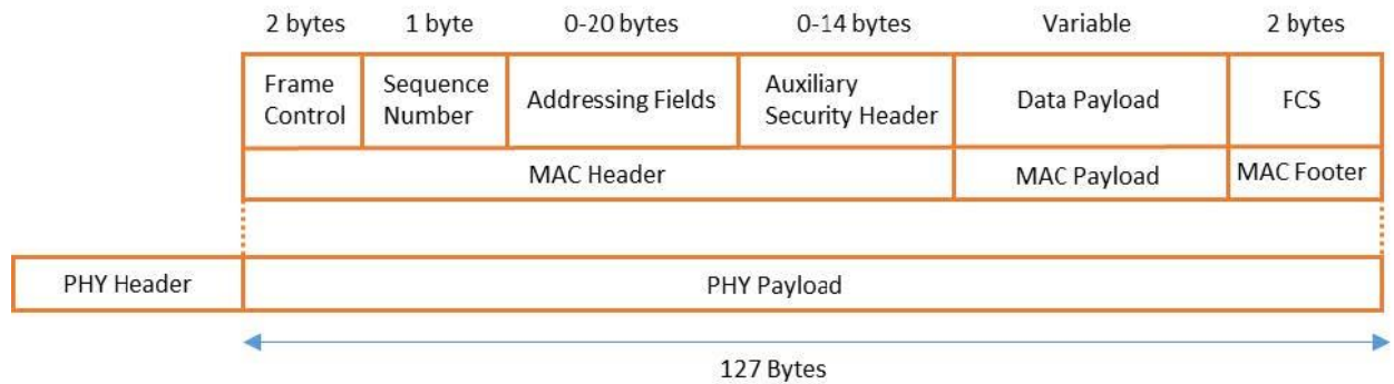
Figure 2. 802.15.4 MAC Payload
