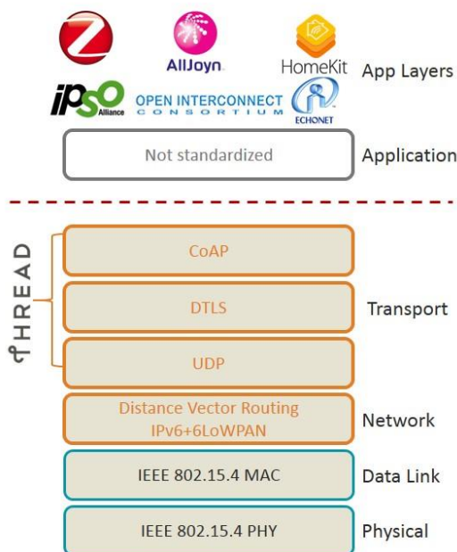
Figure 10. Thread Protocol Layers
