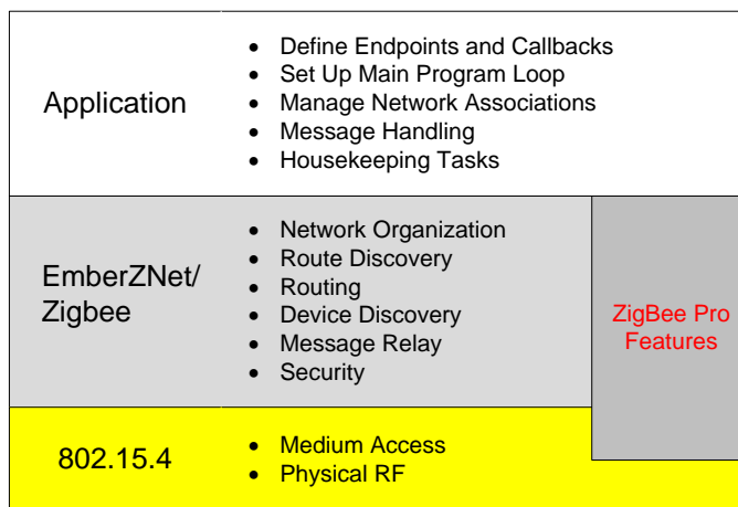
Figure 1. Generic Application Tasks
